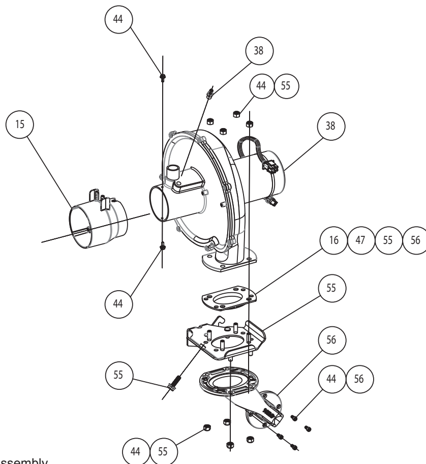
Blower Assembly
