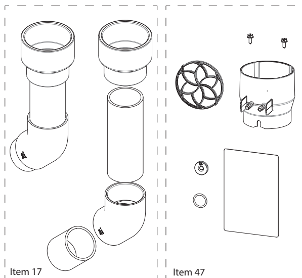
Intake Kit (#17) &amp; Blower Gasket (#47)
