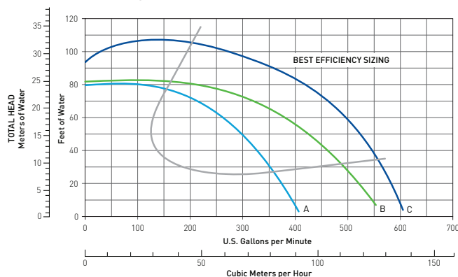
Single Phase Pumps - EQ Models
