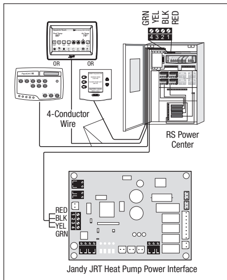
Figure 12. Jandy JRT Heat Pump to Power Center - RS485 (4 wire) connection
