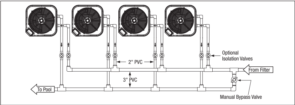
Figure 7. Four (4) Heat Pump Plumbing Layout
