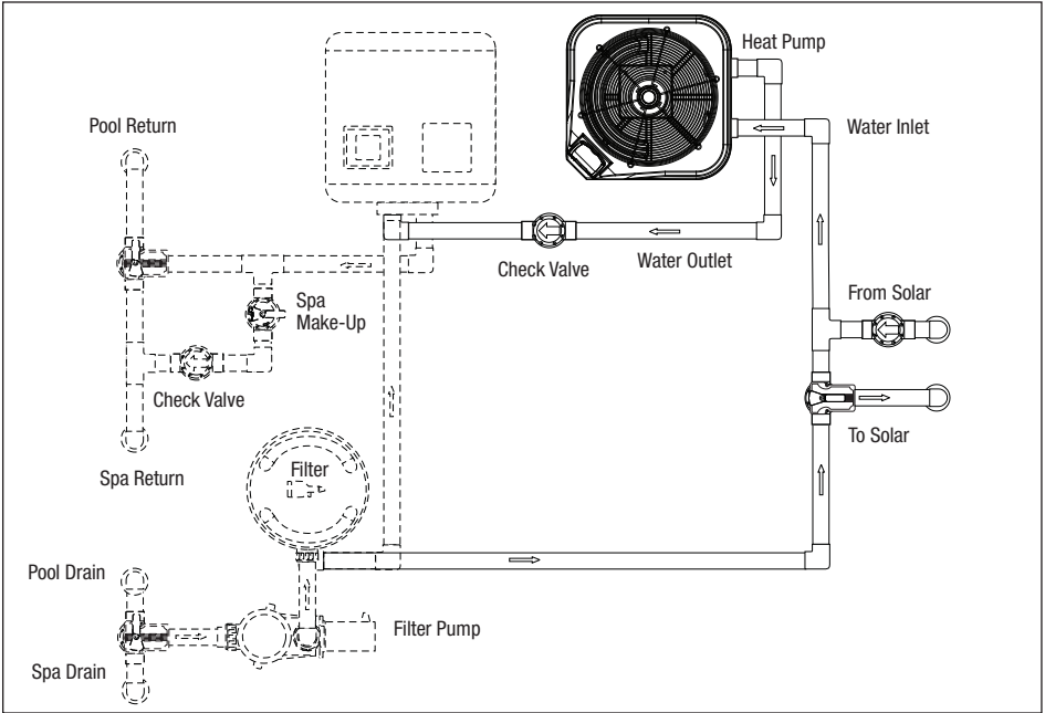
Figure 5. Plumbing for Heating System Combinations
