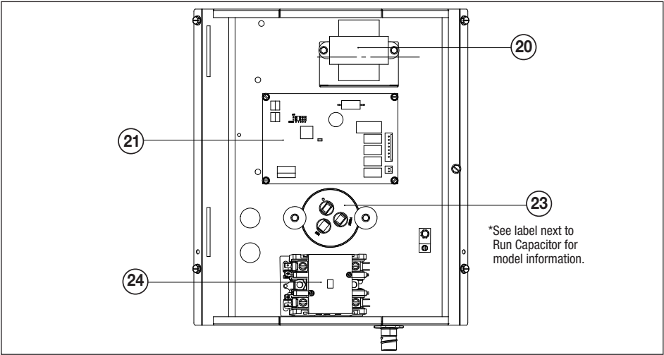
Figure 16. Jandy JRT Single Phase Electric Box
