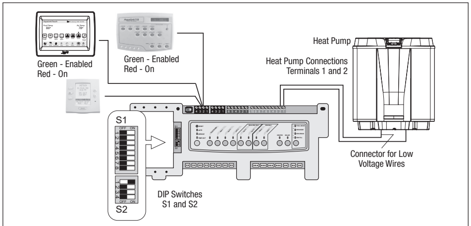
Figure 11. AquaLink RS to Jandy JRT Heat Pump - T-Stat (2 wire) connection
