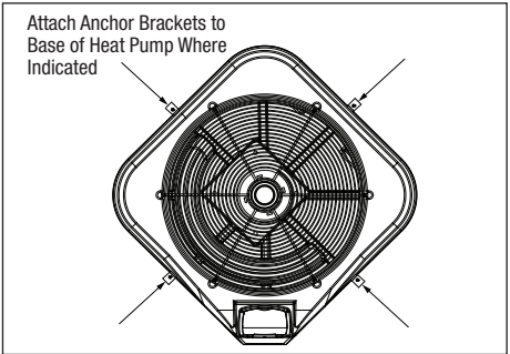
Figure 2. Anchor Clamp Positions
