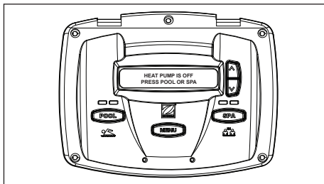
Figura 13. Panel de control principal
