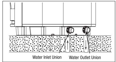
Figure 14. Winterizing the JRT Heat Pump
