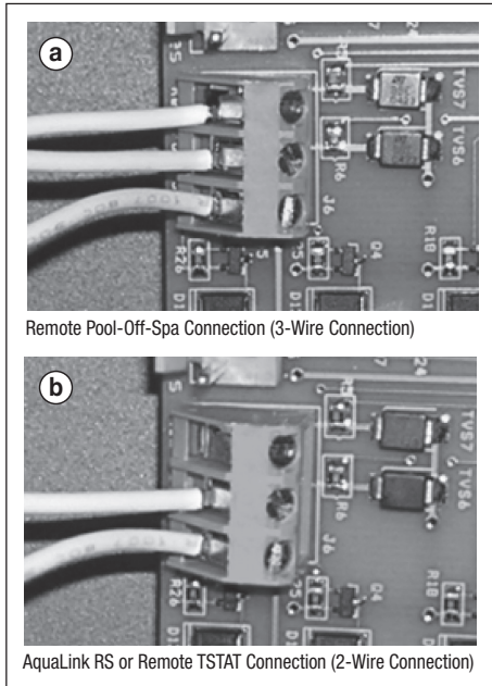
Figure 10. Remote Control Wiring
