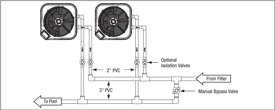
Figure 6. Two (2) Heat Pump Plumbing Layout
