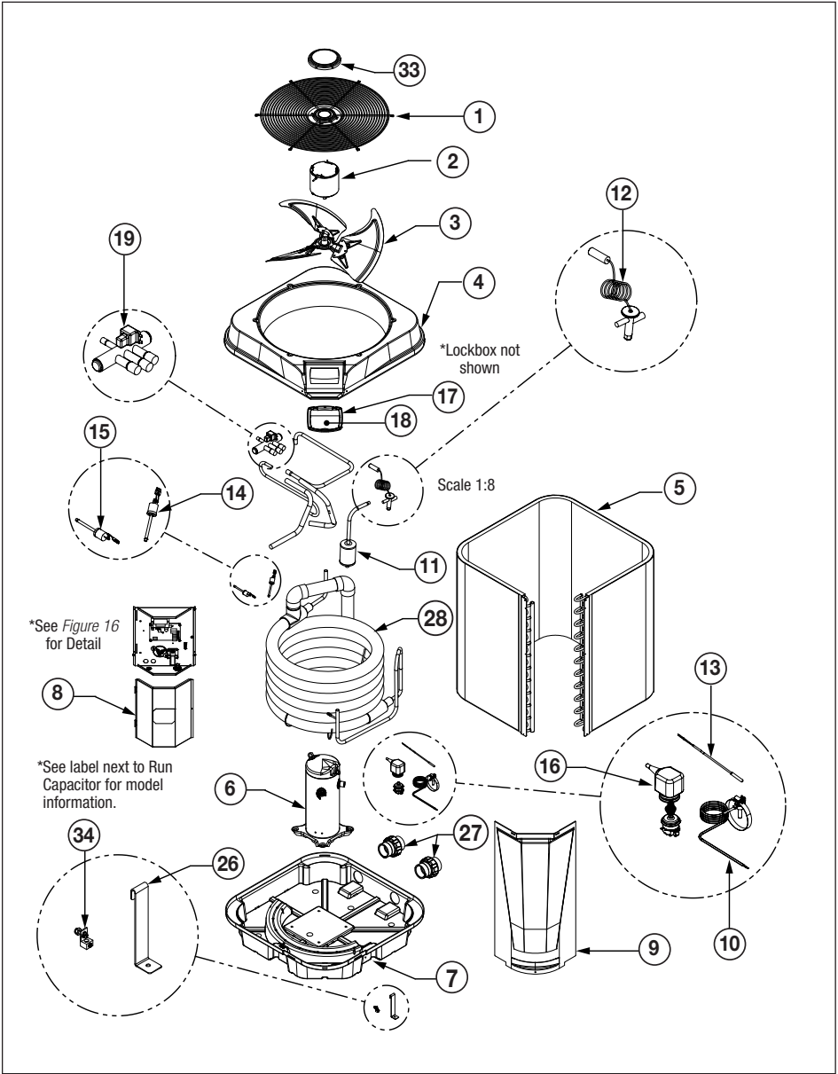
Figure 15. Jandy JRT Heat Pumps Exploded View (JRT2000R Shown)
