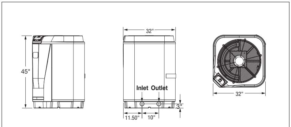
Figure 1. Jandy JRT Heat Pump Dimensions
