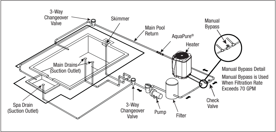
Figure 4. Standard Pumping Layout
