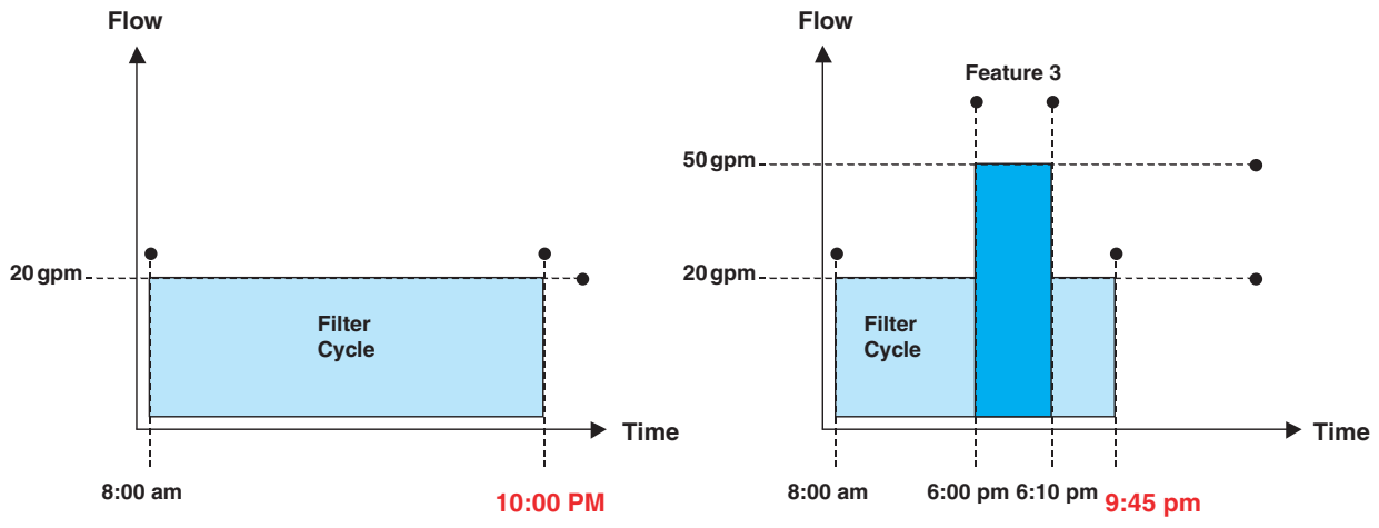
Original Filter Cycle w/No Timed Feature
