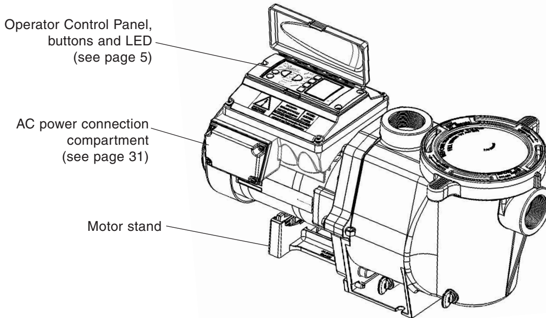
IntelliFlo Drive Assembly
