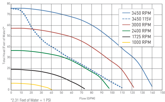
TRISTAR VS 900 PERFORMANCE COMPARISON
