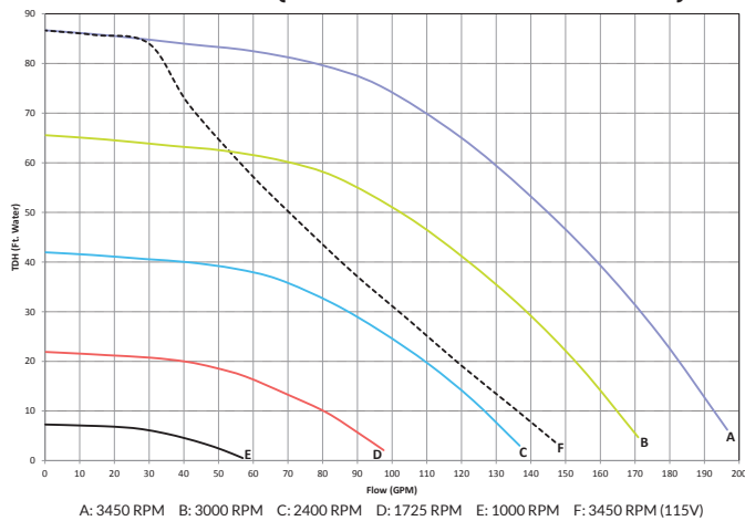
HCP 2500 VS (2.7 HP PERFORMANCE DATA)
