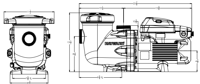
DIMENSIONS (INCHES)
